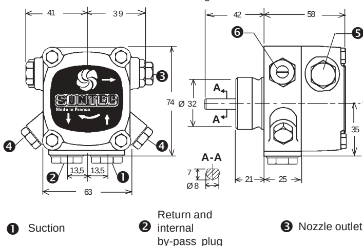
Hub mounting
