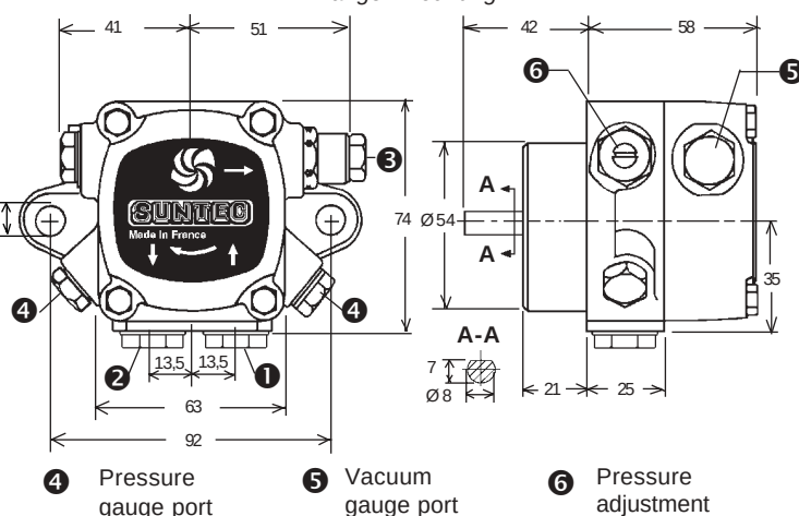
Flange mounting
